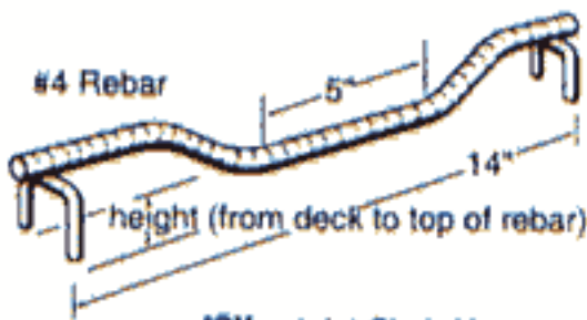
JCU —Joist Chair Upper
